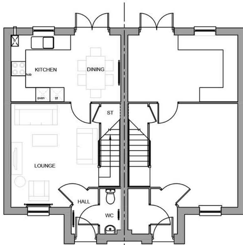
GROUND FLOOR PLAN Palmerston (end)
